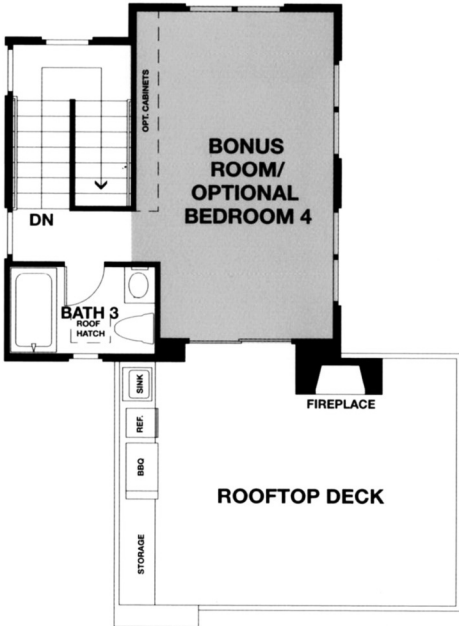
THIRD FLOOR
